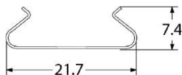
Clip incasso Recessed clip
