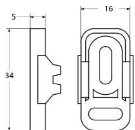
Clip fissa Fixed Clip
